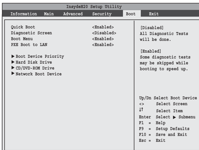
Figure 13. Boot Menu
